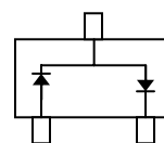
TOP VIEW BAT54SW
