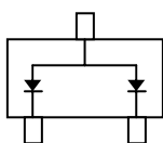
TOP VIEW BAT54AW
